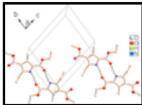
Fig. 2. Dimer formation in the crystal packing.
