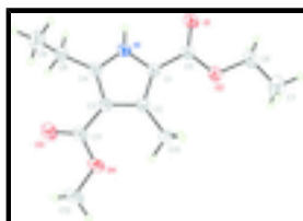
Fig. 1. Molecular structure with the unique atom-labelling scheme. Displacement ellipsoids are drawn at the 30% probability level.
